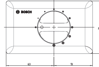
Dimensions LM1-VC36P
