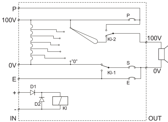
LM1-VC12P/L
