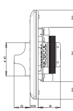
Dimensions LM1-VC36P
