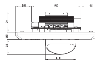
Dimensions LM1-VC36L
